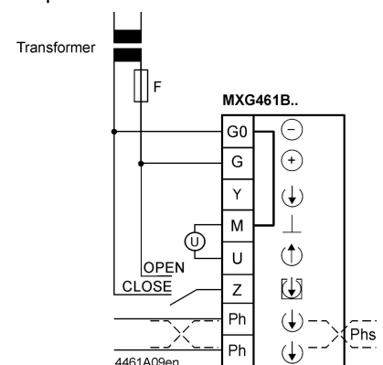
Separate Transformer
