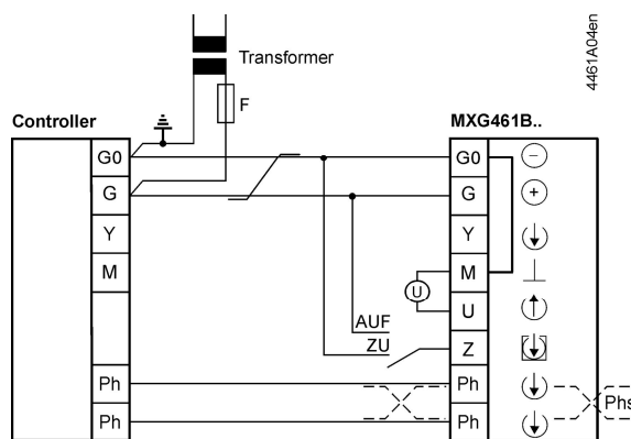
Common Transformer
