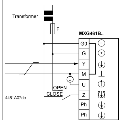
Separate Transformer
